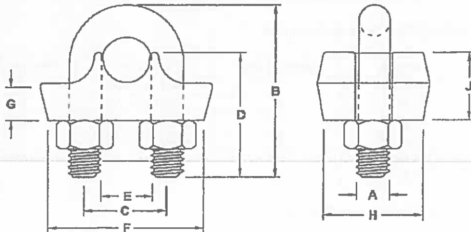
Fig. 5: Bull Dog type connector.
