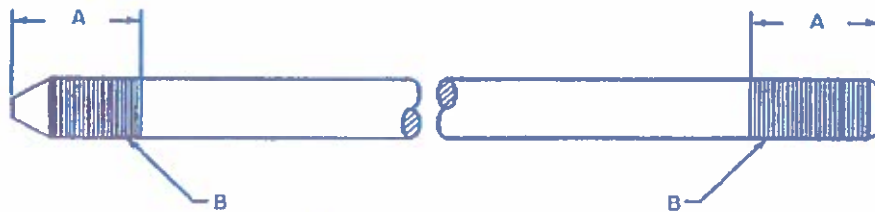
Fig. 1: Threading dimensions
